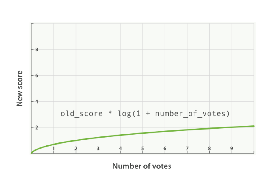
Figure 17-4. Logarithmic popularity based on an original_score of 2.0
