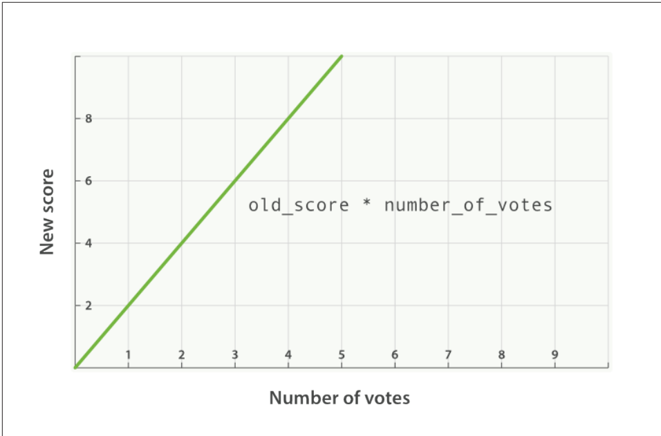
Figure 17-3. Linear popularity based on an original _score of 2.0
