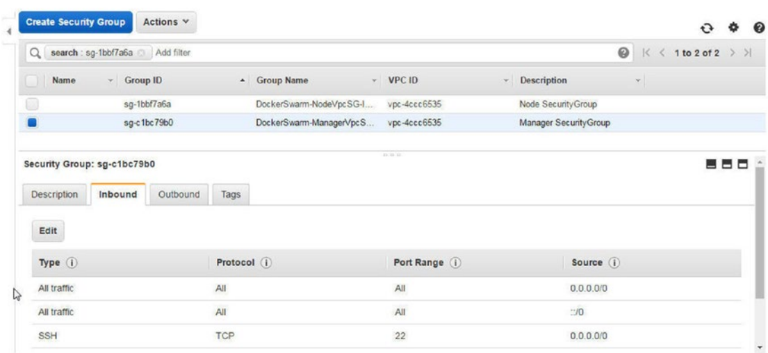
Figure 15-6. The security group inbound rules are enabled for all traffic
