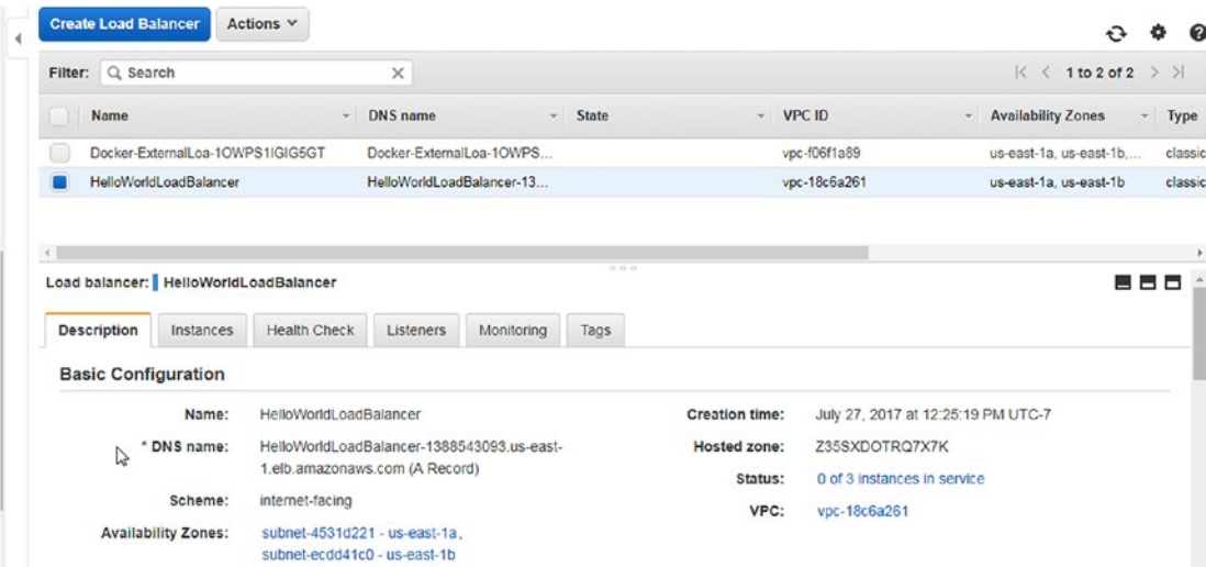
Figure 12-17. Obtaining the DNS name of the load balancer
