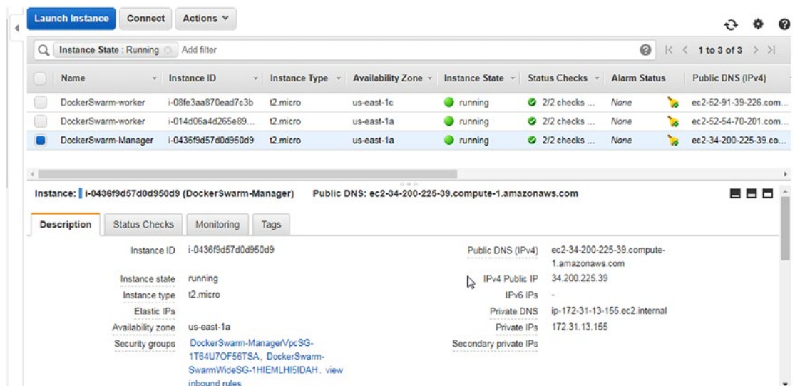
Figure 4-3. EC2 instances for Swarm
