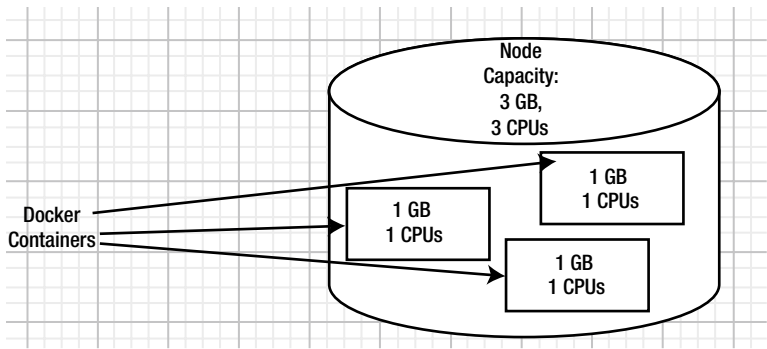
Figure 7-5. Resource allocation with resource reserves set
