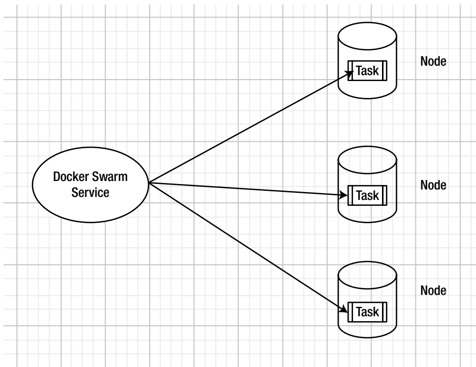
Figure 8-3. Using the spread scheduling policy
