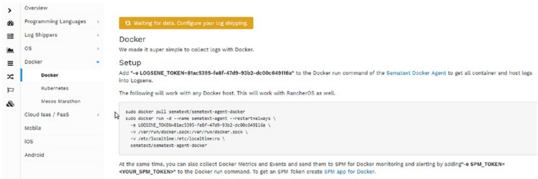
Figure 11-9. The Logsene app is added and LOGSENE_TOKEN is generated
