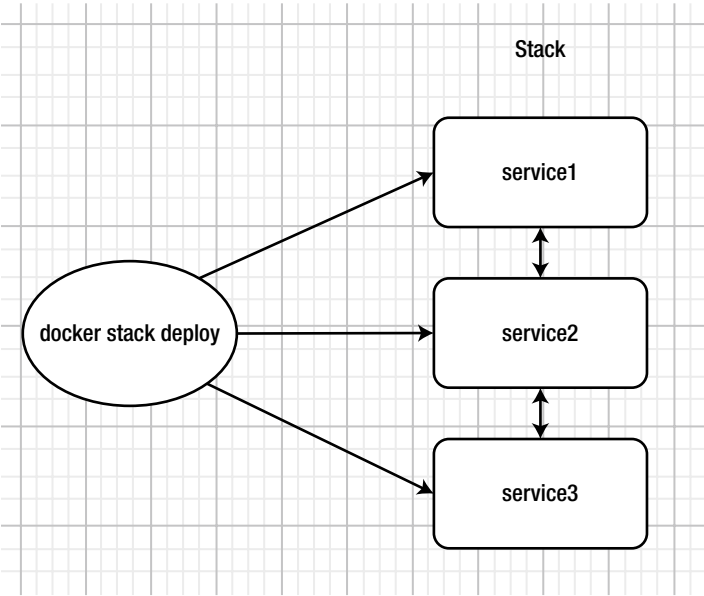
Figure 15-1. Service stack created with the docker stack deploy command
