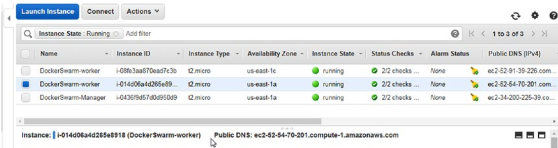
Figure 4-7. Obtaining the public DNS for a EC2 instance on which a Swarm worker node is hosted
