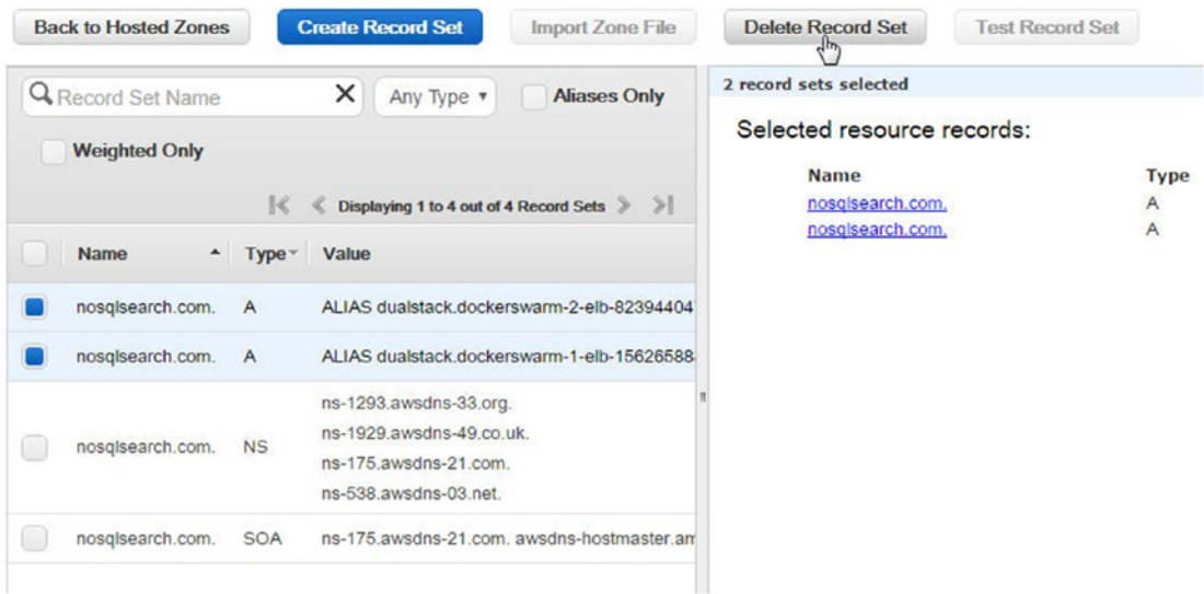
Figure 13-41. Deleting the record sets
