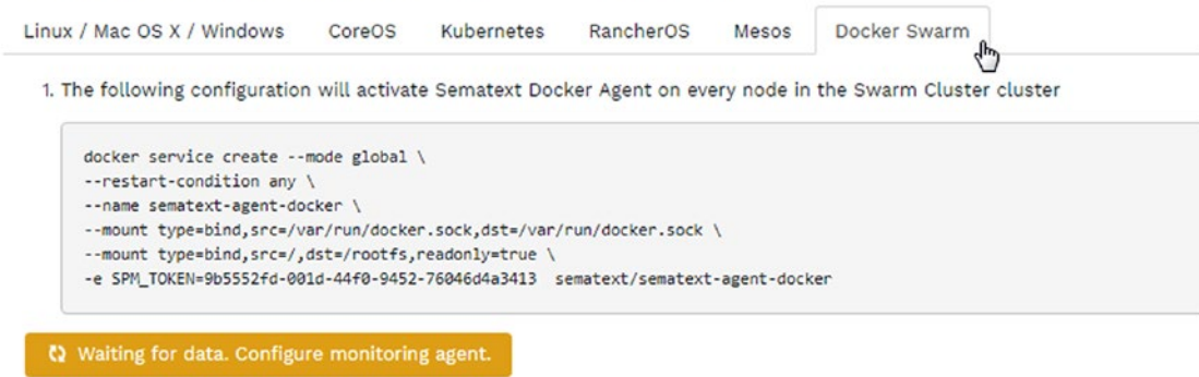
Figure 11-4. Docker Swarm configuration
