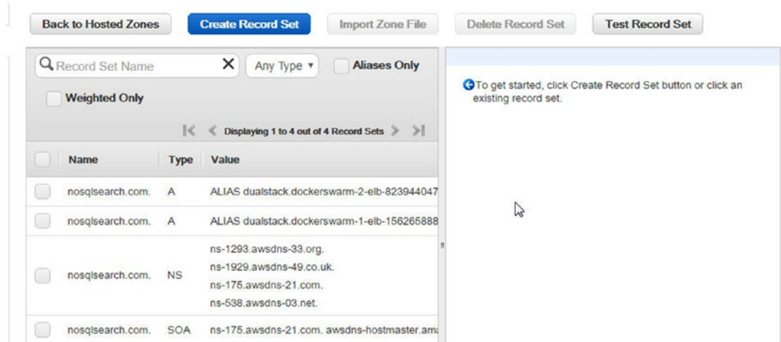
Figure 13-34. Secondary record set is created
