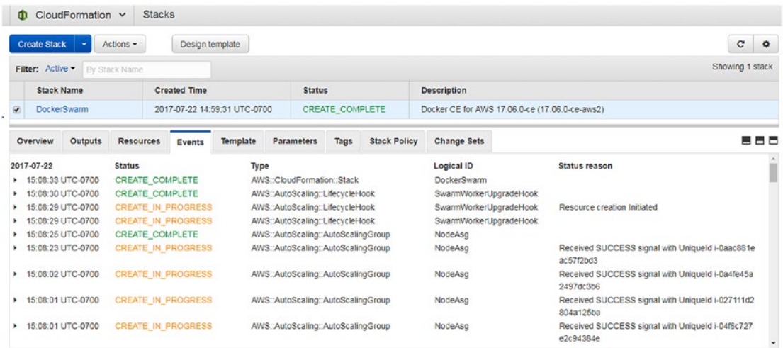
Figure 3-17. Stack status is CREATE_COMPLETE
