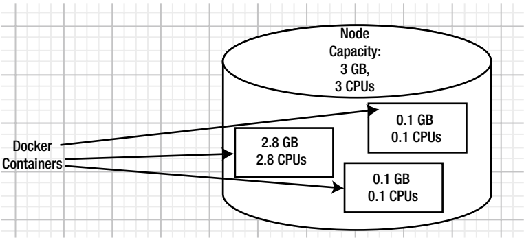
Figure 7-2. Unequal allocation of resources
