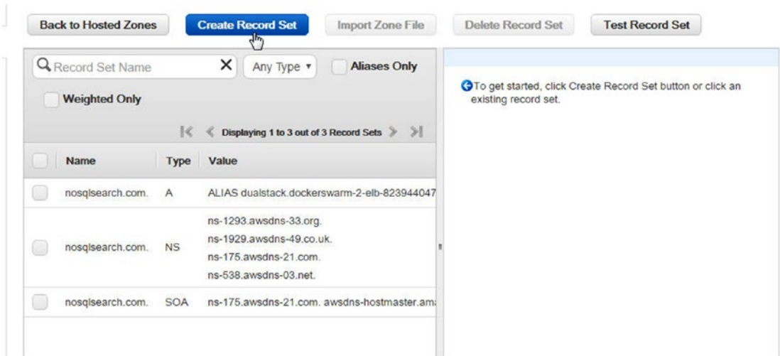
Figure 13-30. Creating another record set
