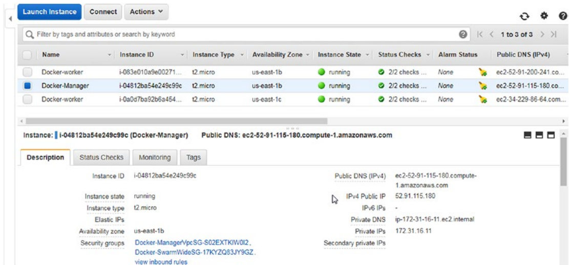
Figure 7-7. EC2 instances for Swarm nodes
