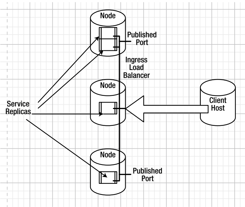
Figure 12-1. Ingress load balancing
