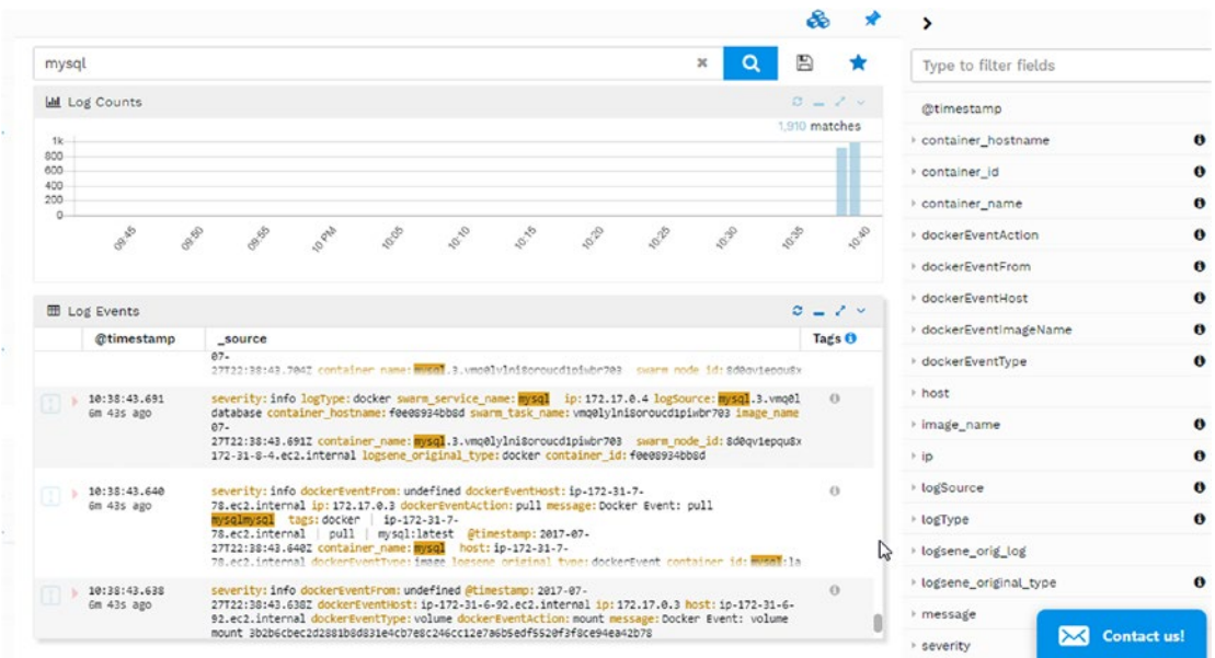
Figure 11-20. Logs for Docker event for mysql image pull
