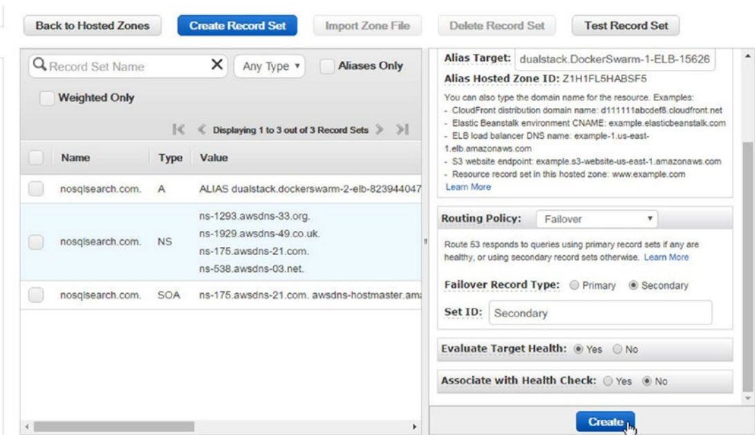
Figure 13-33. Creating a secondary record set
