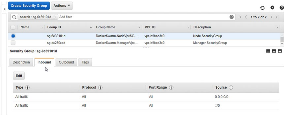
Figure 4-4. Setting inbound rules on a security group to allow all traffic
