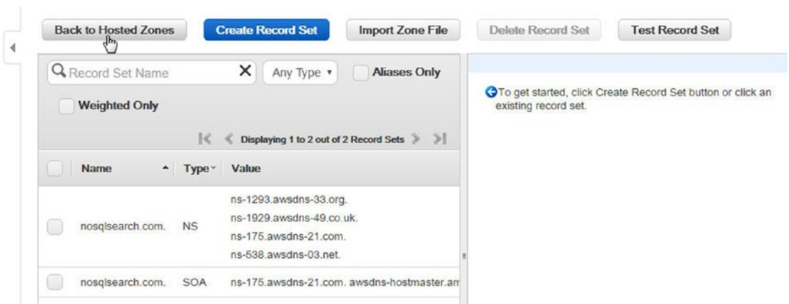
Figure 13-43. Going back to the hosted zones
