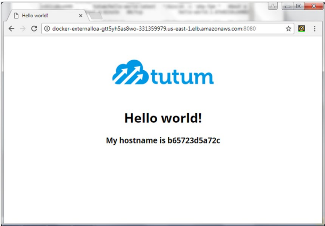
Figure 10-5. Invoking a Docker service in the ingress network using EC2 elastic load balancer public DNS
