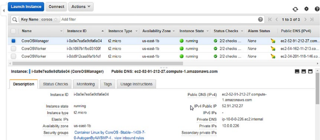
Figure 12-3. CoreOS instances on EC2 for a manager and two worker nodes
