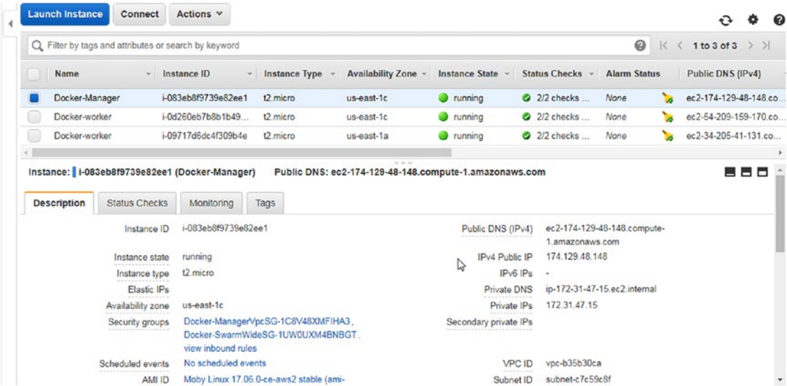
Figure 10-4. Obtaining the public IP address of a Swarm manager node instance
