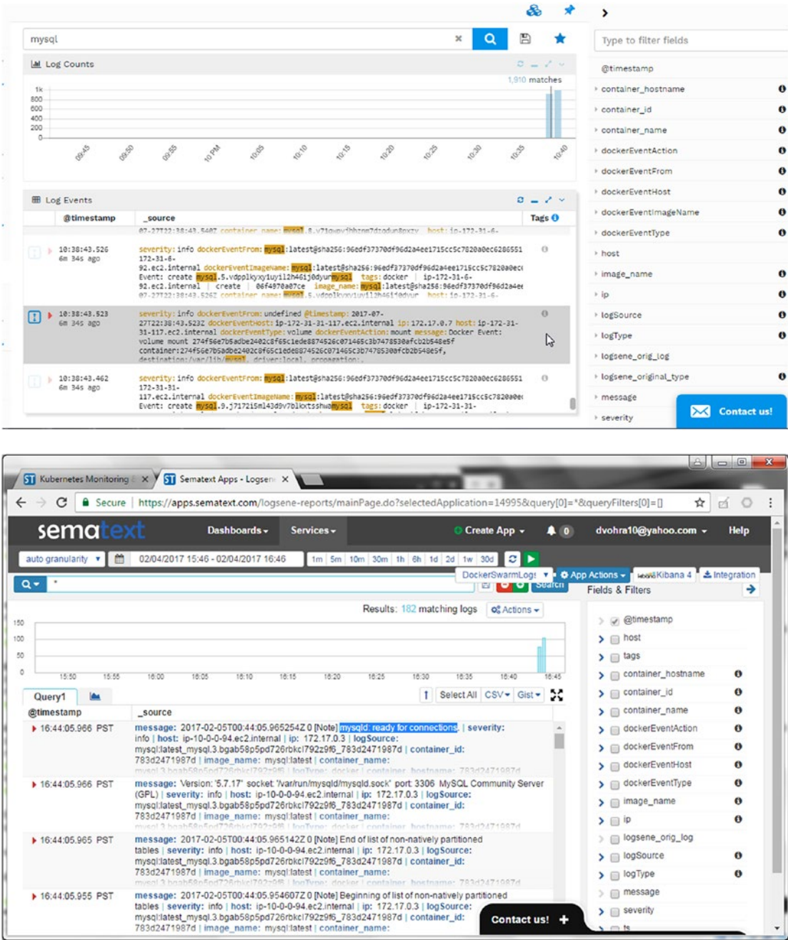
Figure 11-21. Logs for Docker event volume mount
