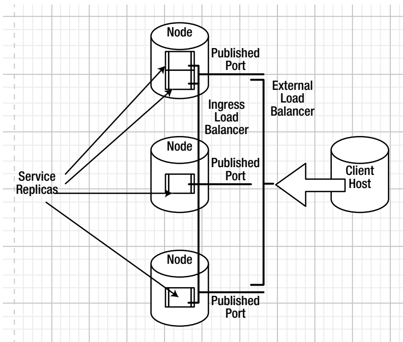
Figure 12-2. External load balancer
