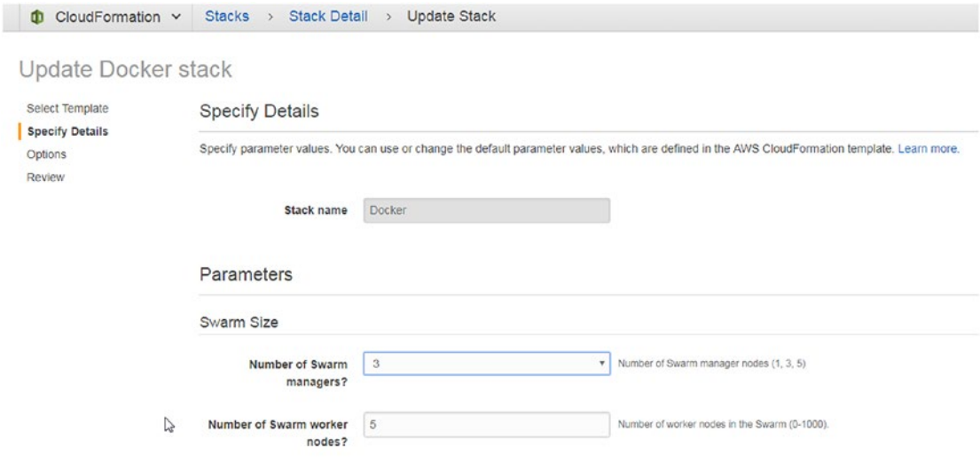
Figure 11-15. Increasing the number of worker nodes
