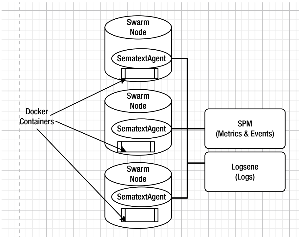
Figure 11-1. Sematext Docker agent on each Swarm node
