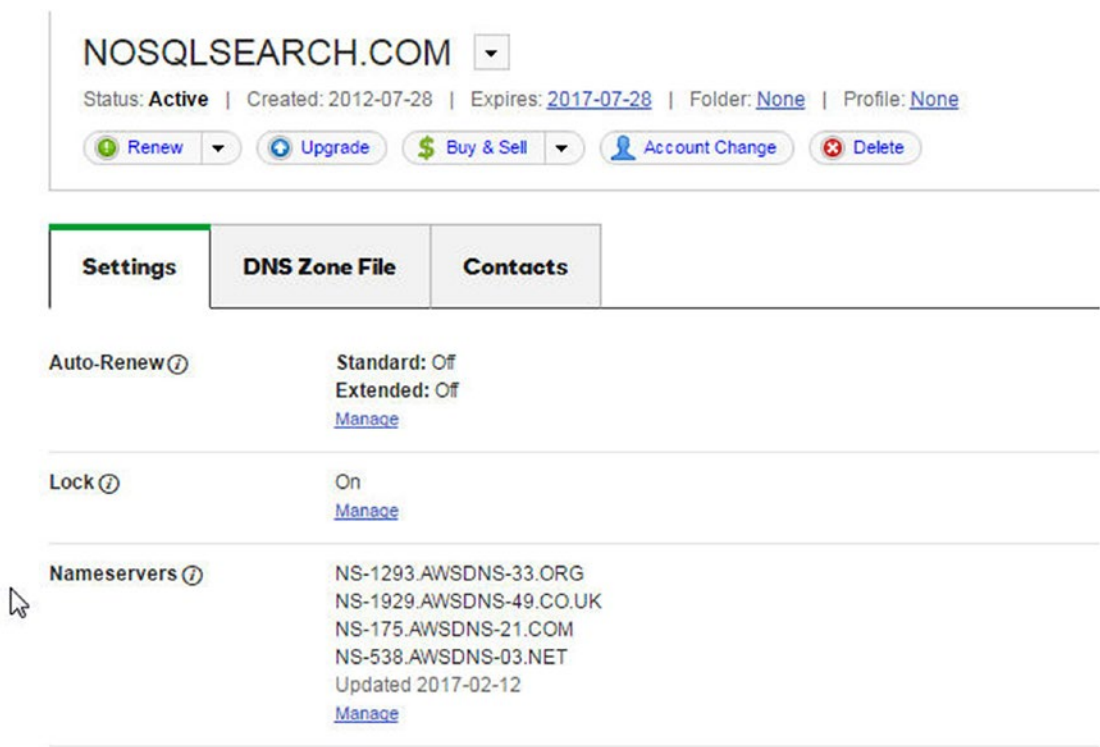
Figure 13-21. Name servers configured on a domain
