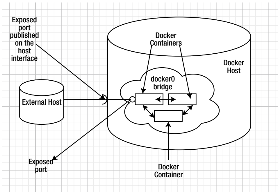
Figure 10-1. The default docker0 bridge network
