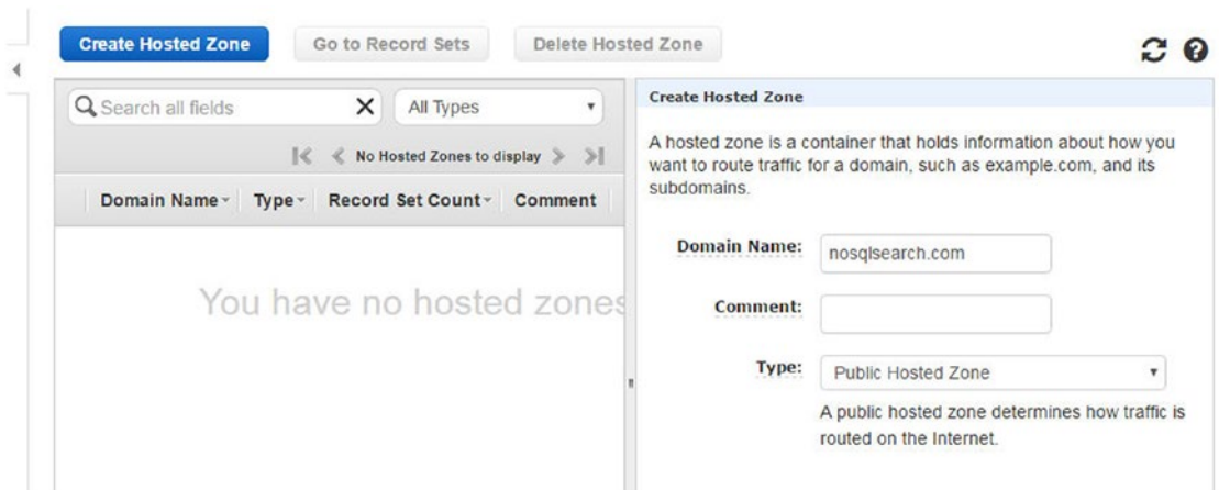
Figure 13-18. Configuring the hosted zone
