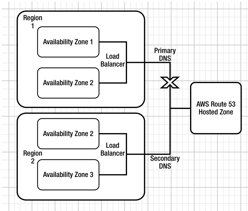
Figure 13-2. Amazon Route 53 provides DNS failover across AWS regions
