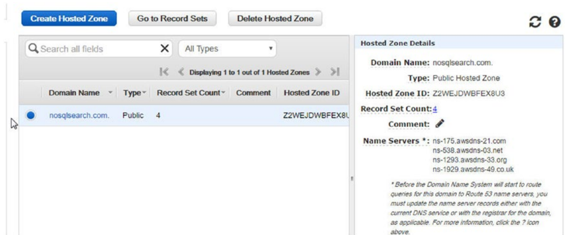
Figure 13-35. Hosted zone created
