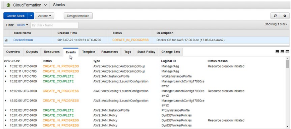
Figure 3-16. CloudFormation stack events
