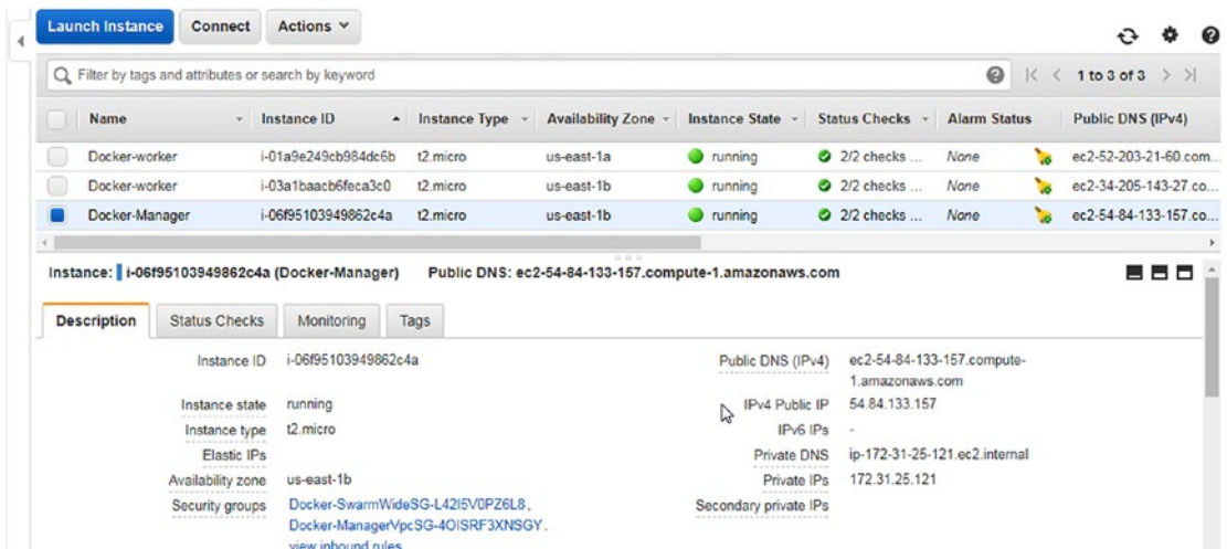
Figure 8-5. EC2 instances for the Docker swarm
