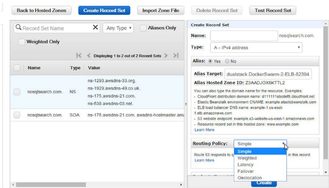
Figure 13-25. Selecting a routing policy
