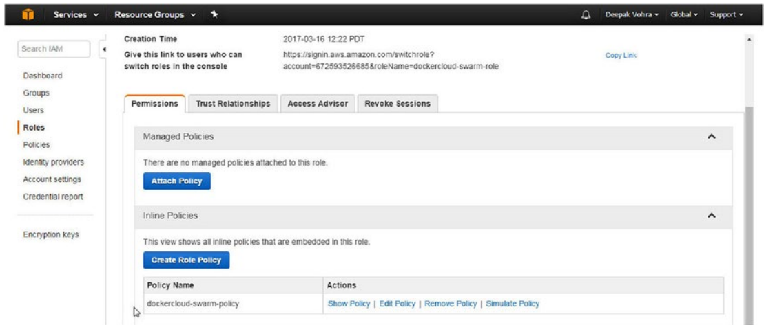
Figure 14-15. The new inline policy is added
