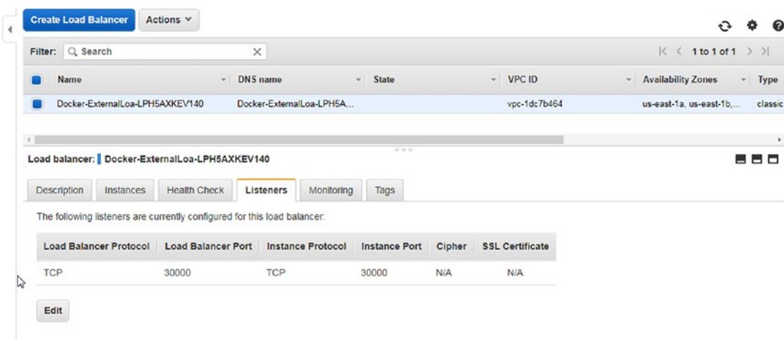
Figure 10-6. Adding a load balancer listener
