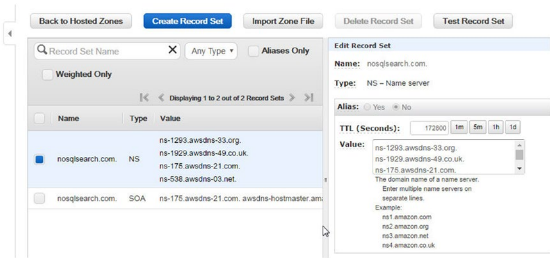
Figure 13-19. The new public hosted zone
