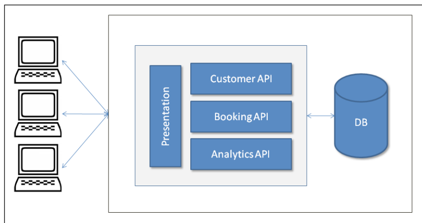
Monolithic design with services
