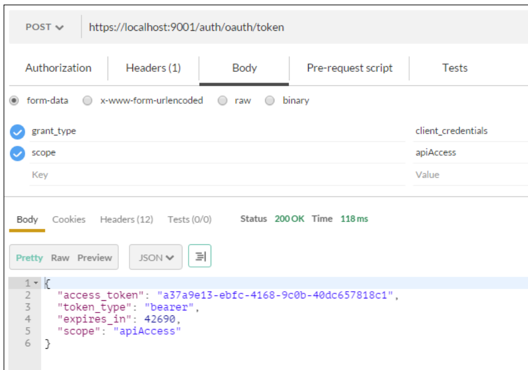
OAuth 2.0 client credentials grant – access token request and response
