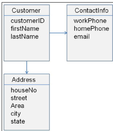
The customer as an aggregate
