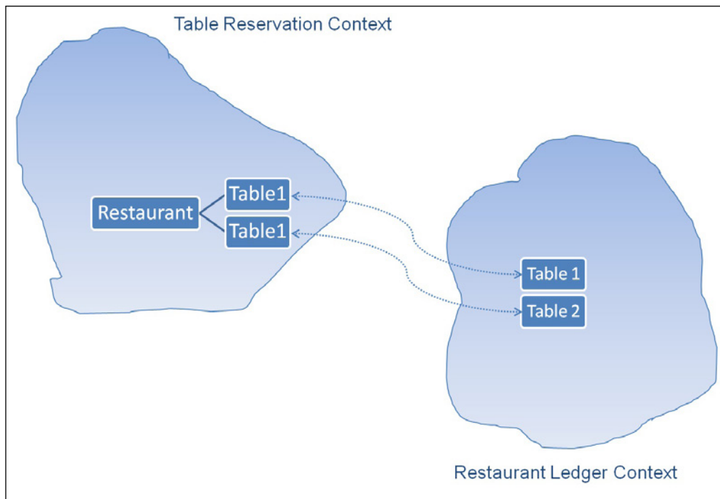
Context map example
