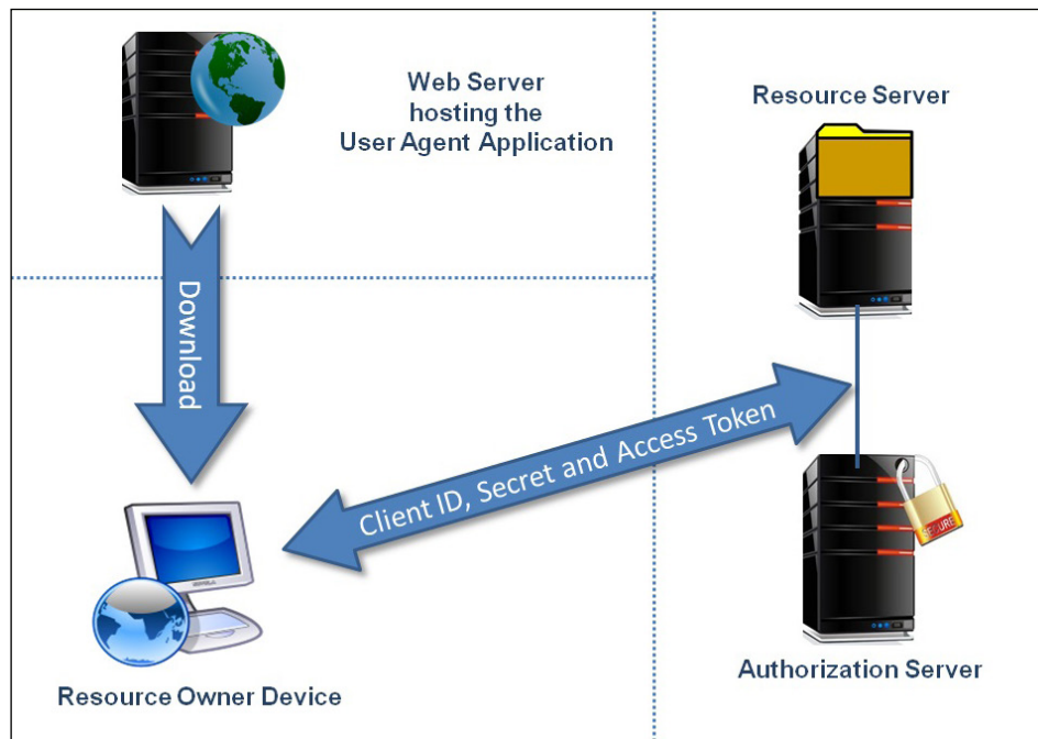
OAuth 2.0 client user agent application profile
