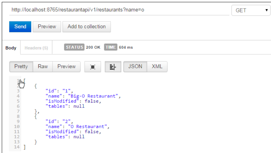
Restaurant Service call using Edge Server
