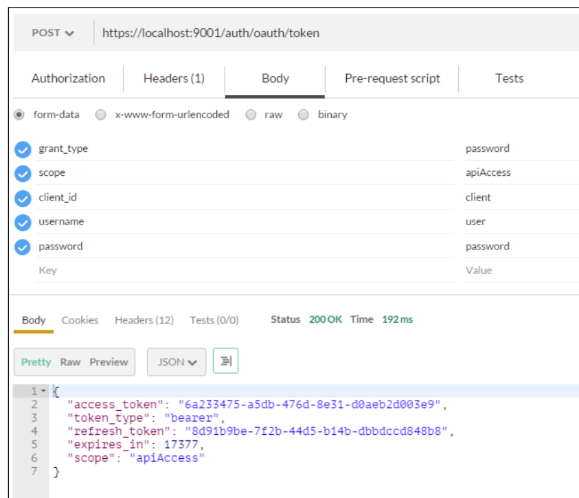
OAuth 2.0 resource owner password credentials grant – access token request and response
