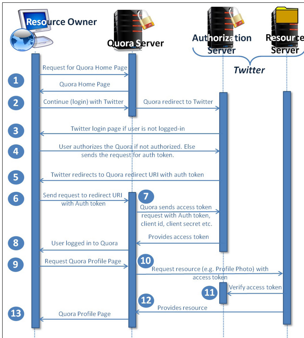
OAuth 2.0 authorization code grant flow
