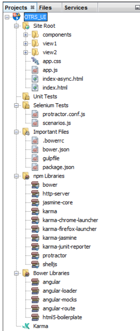
AngularJS seed directory structure
