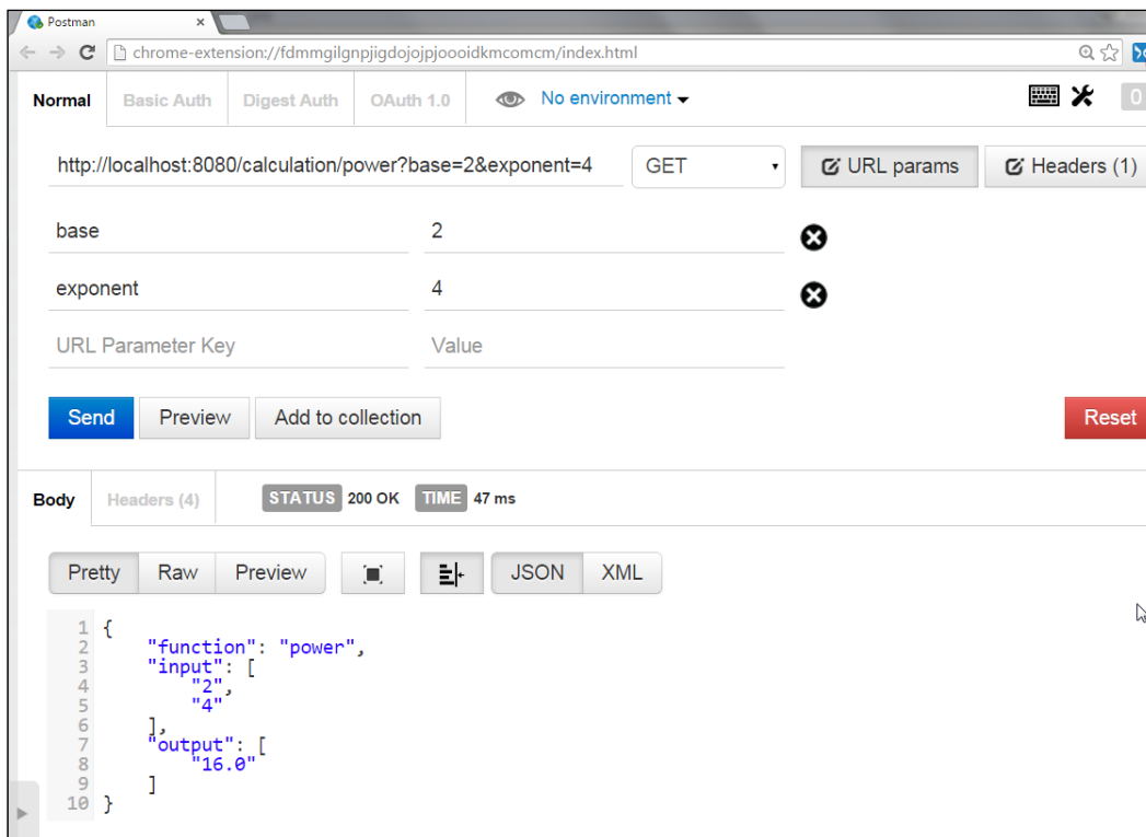
Calculation (power) resource test with Postman
