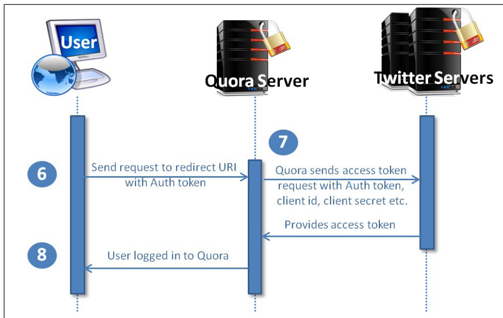
OAuth 2.0 client web application profile
