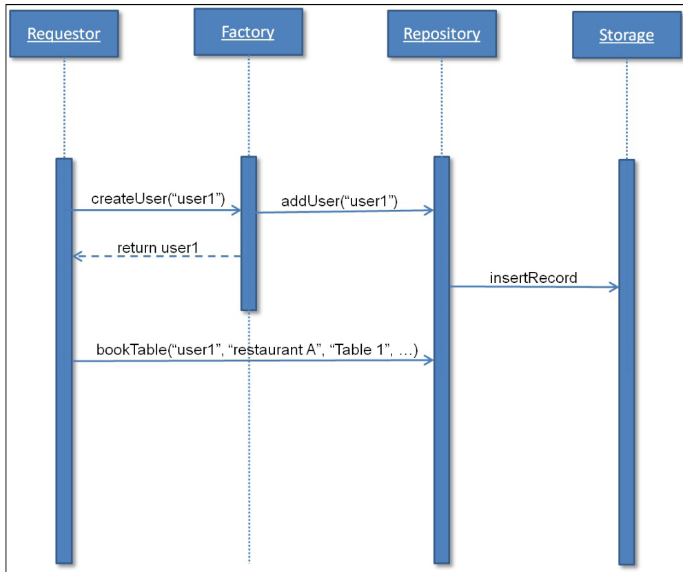
Repository object flow
