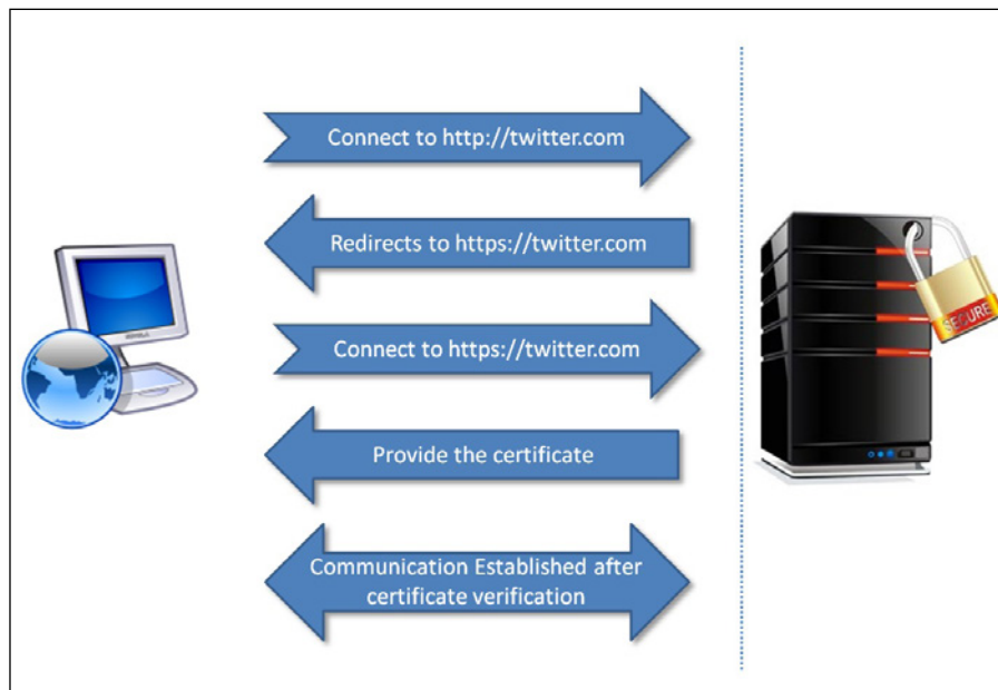
Secure HTTP communication
