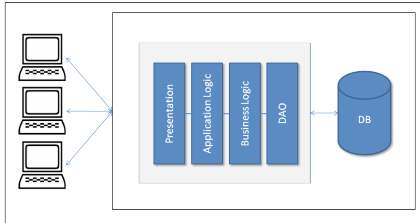
Traditional monolithic design
