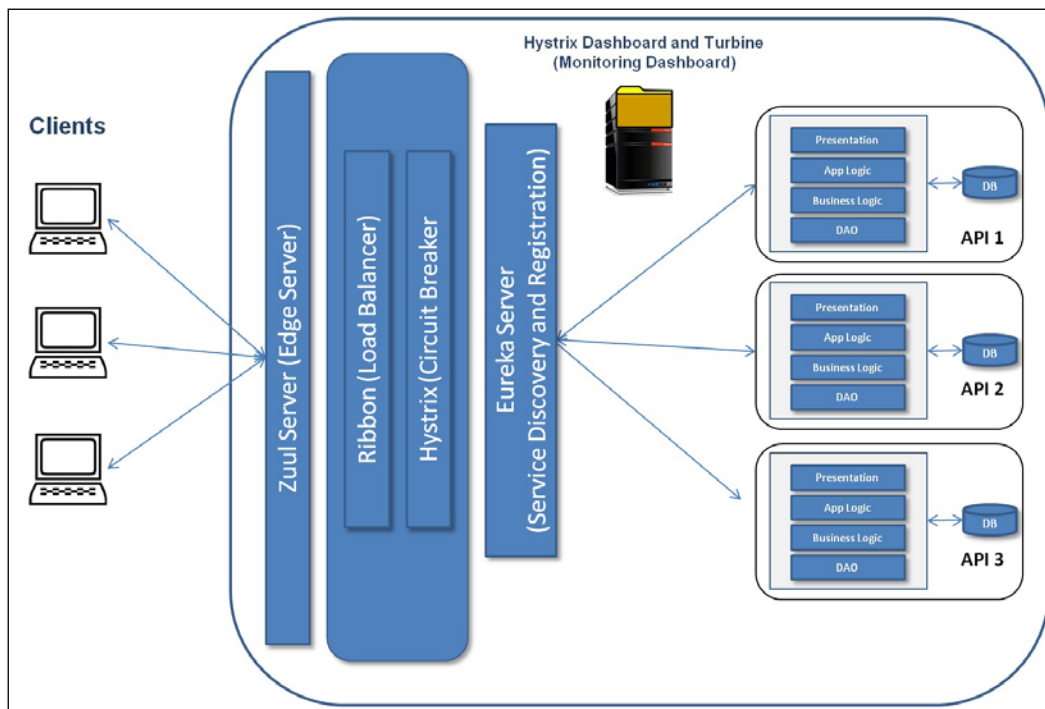
Microservice architecture diagram
