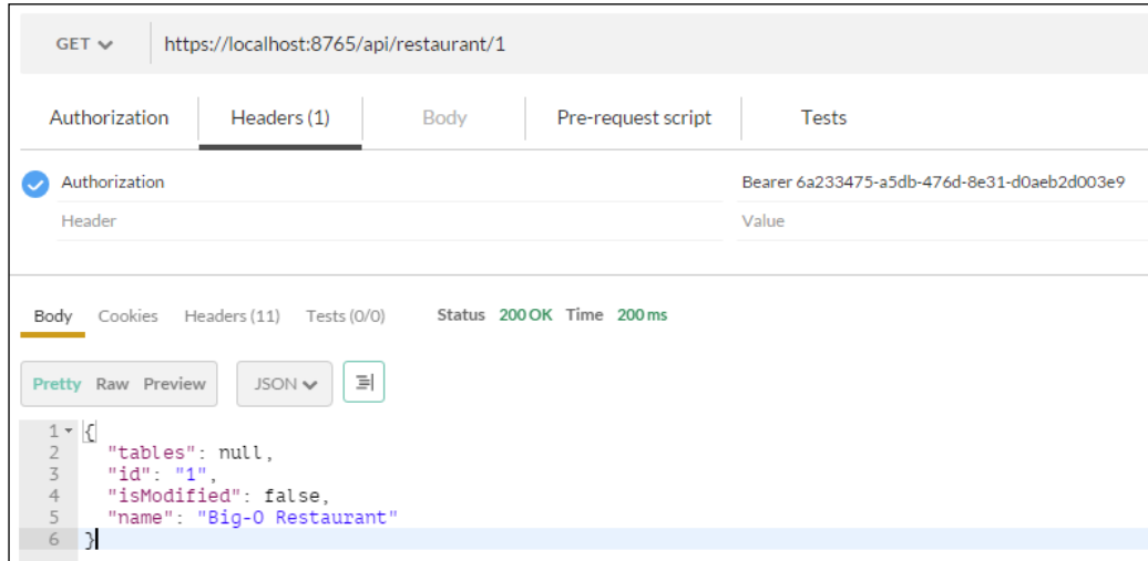
OAuth 2.0 authorization code grant – using the access token for API access
