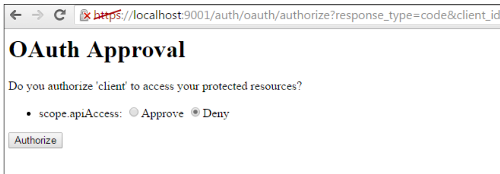
OAuth 2.0 authorization code grant – resource grant approval
