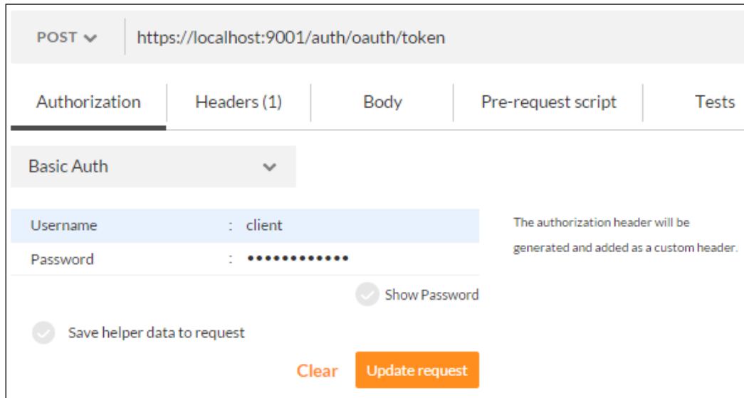
OAuth 2.0 authorization code grant – access token request – adding the authentication
