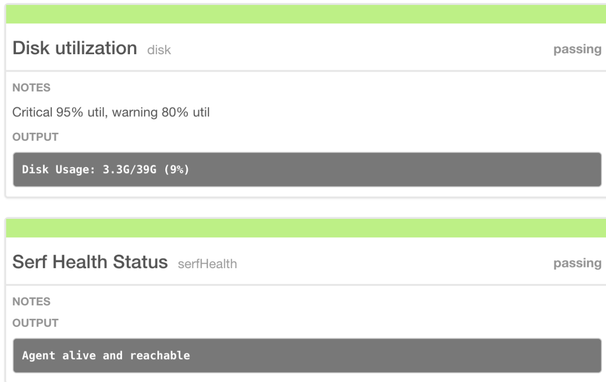
Figure 15-15: Hard disk checks in Consul UI
