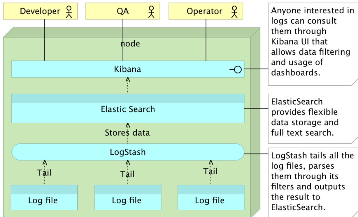
Figure 16-02: ELK stack running on a single server
