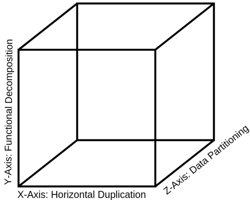
Figure 14-1: Scale cube
