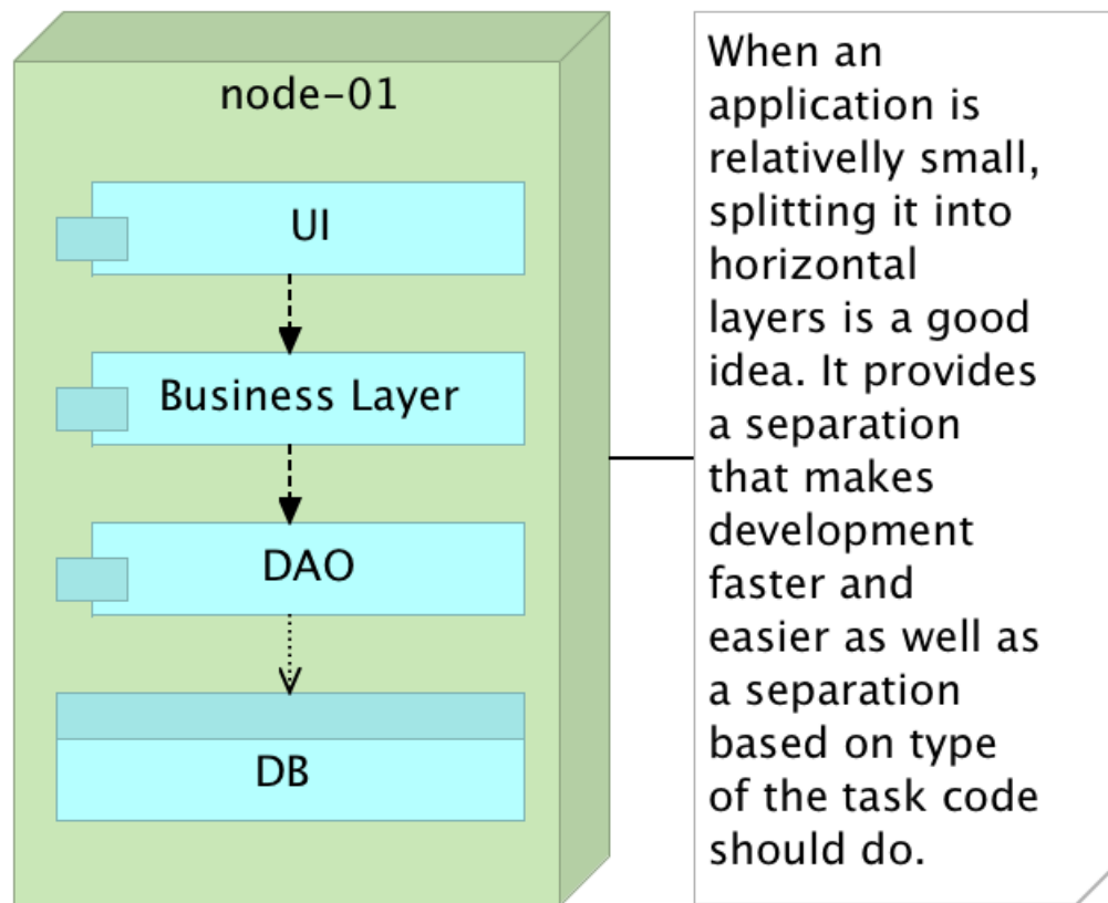
Figure 3-1: Monolithic application
