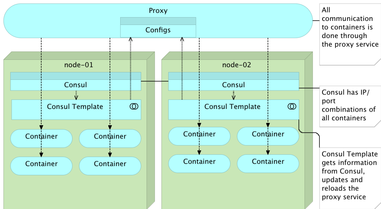
Figure 9-3: Services with automatic proxy with Consul Template
