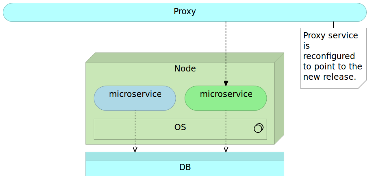
Figure 13-4: Proxy is re-configured to point to the new release
