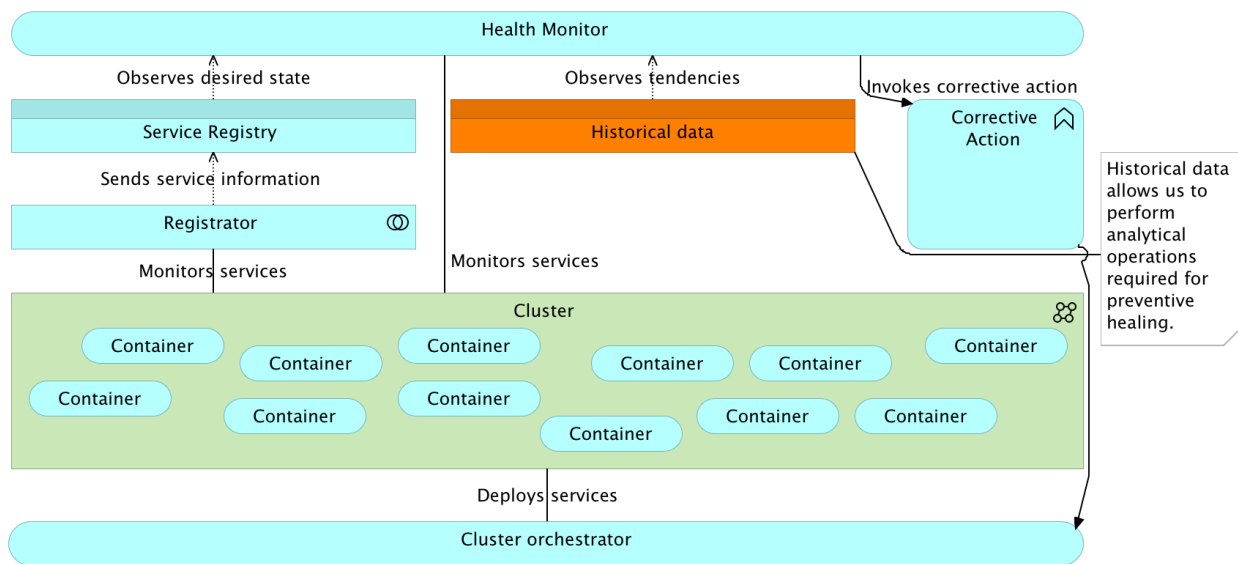
Figure 15-11: Self-healing system architecture: Preventive healing requires historical data to be analyzed
