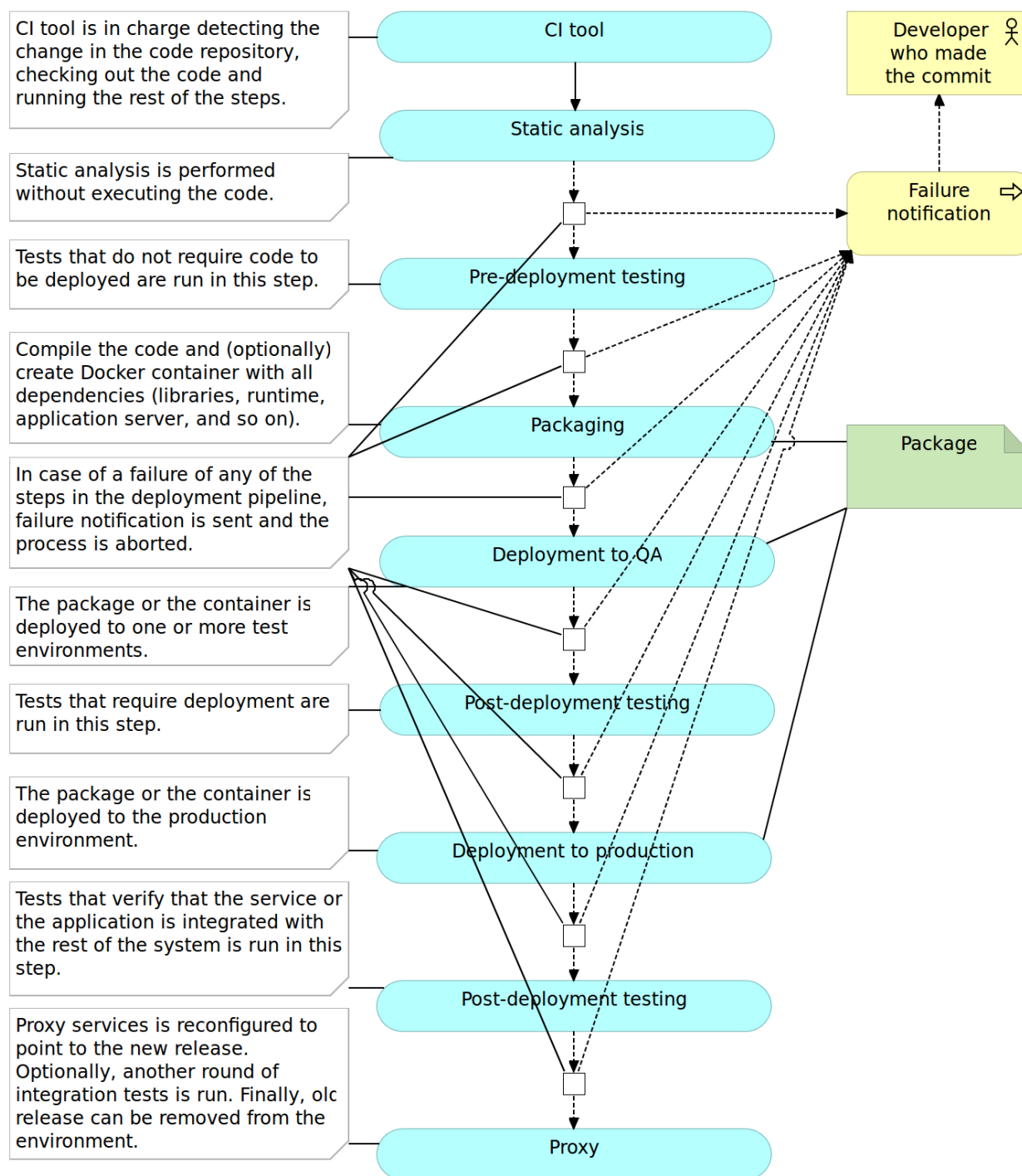
Figure 2-7: Continuous deployment pipeline
