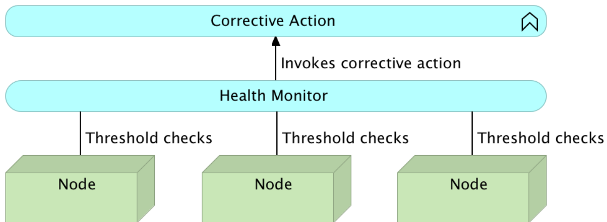
Figure 15-03: Hardware level self-healing
