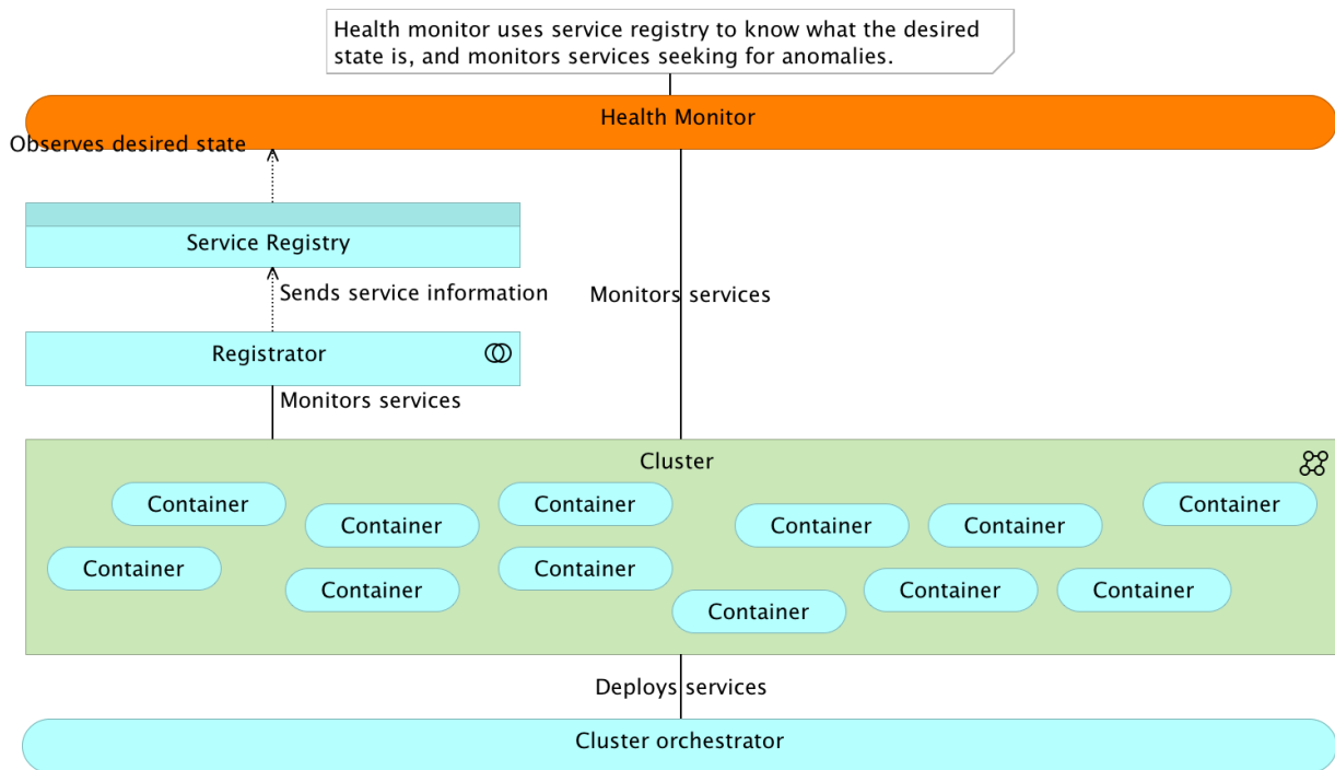
Figure 15-09: Self-healing system architecture: With all the relevant information stored in a service registry, some health monitoring tools can utilize it to verify whether the desired state is maintained
