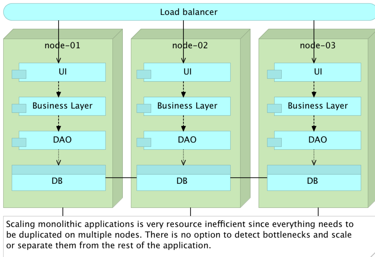
Figure 14-2: Monolithic application scaled inside a cluster
