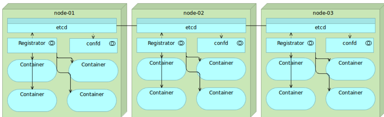
Figure 8-8: Multiple nodes with Docker containers, etcd, Registrator and confd
