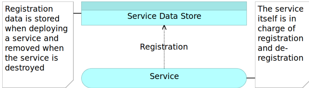
Figure 8-4: Self-registration
