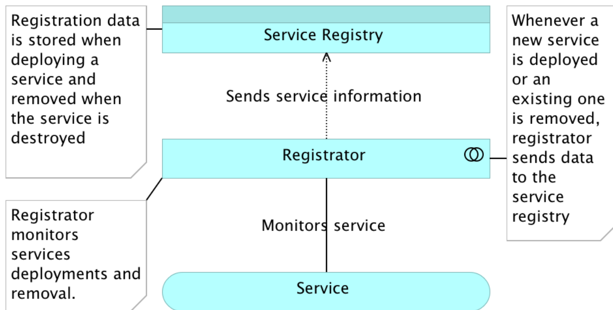
Figure 8-5: Registration service
