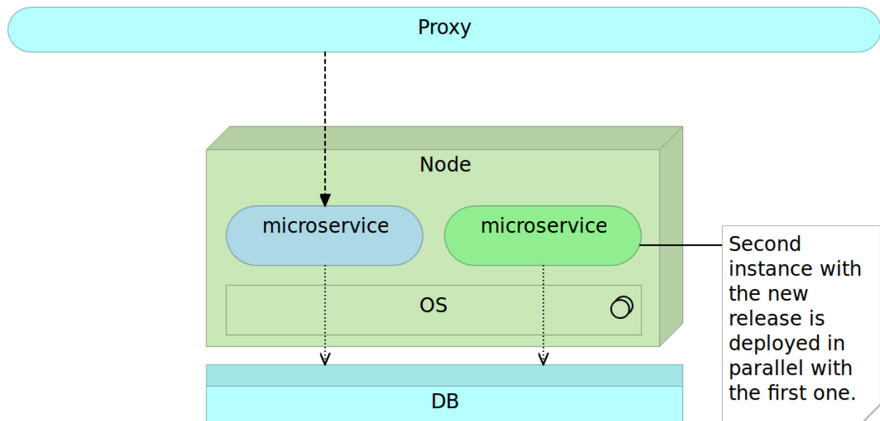
Figure 13-3: New release of the immutable microservice deployed alongside the old release
