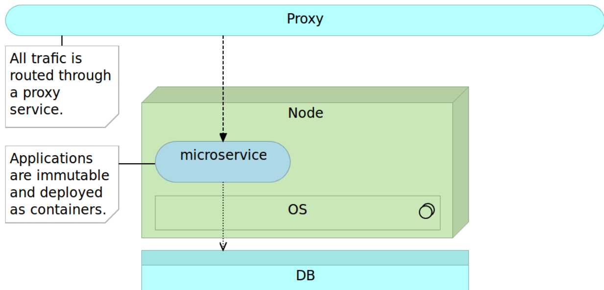
Figure 13-2: Immutable microservice deployed as a container
