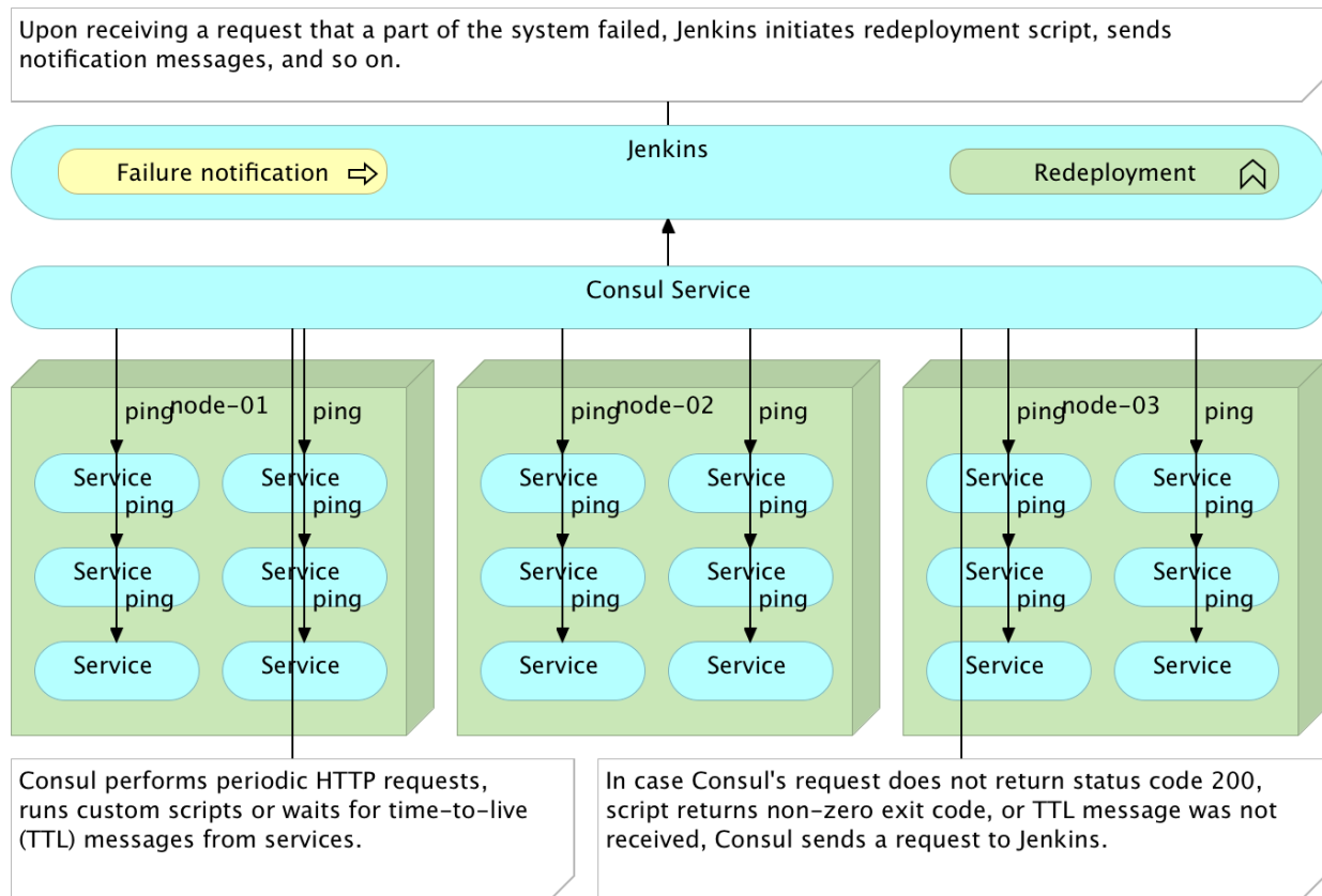
Figure 15-20: Checking and healing Consul pinging services
