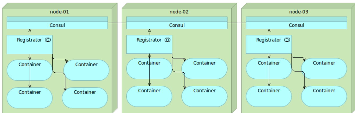
Figure 8-10: Multiple nodes with Docker containers, Consul and Registrator
