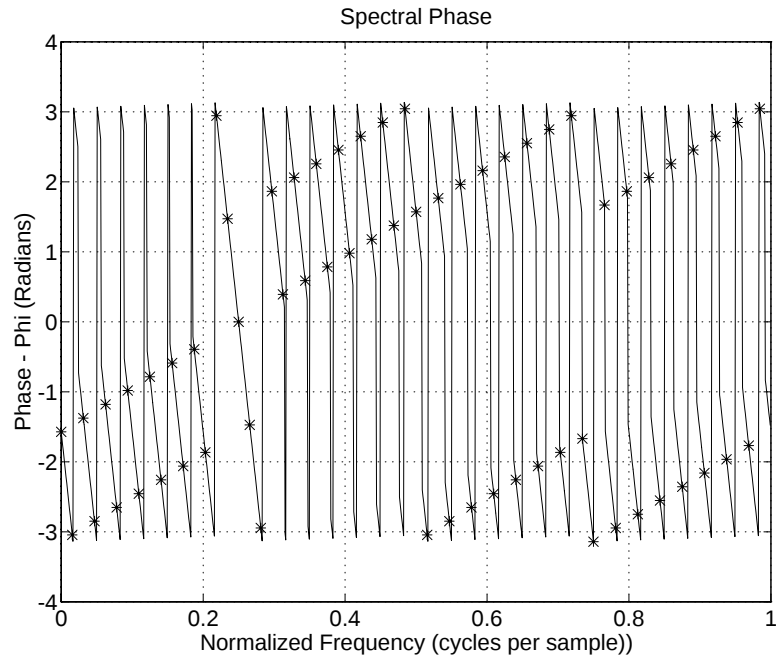
Figure 9.10: Spectral phase.
