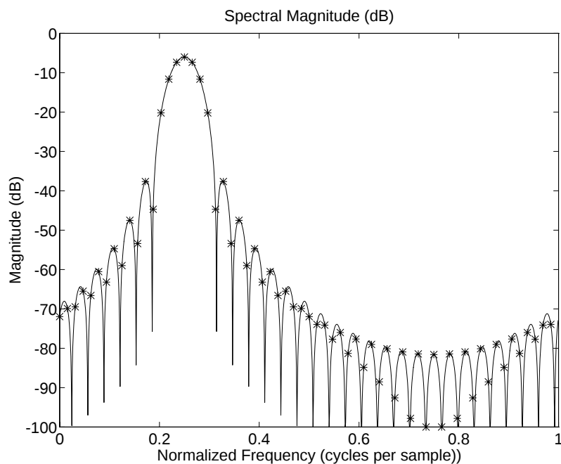
Figure 9.9: Spectral Magnitude, dB scale.
