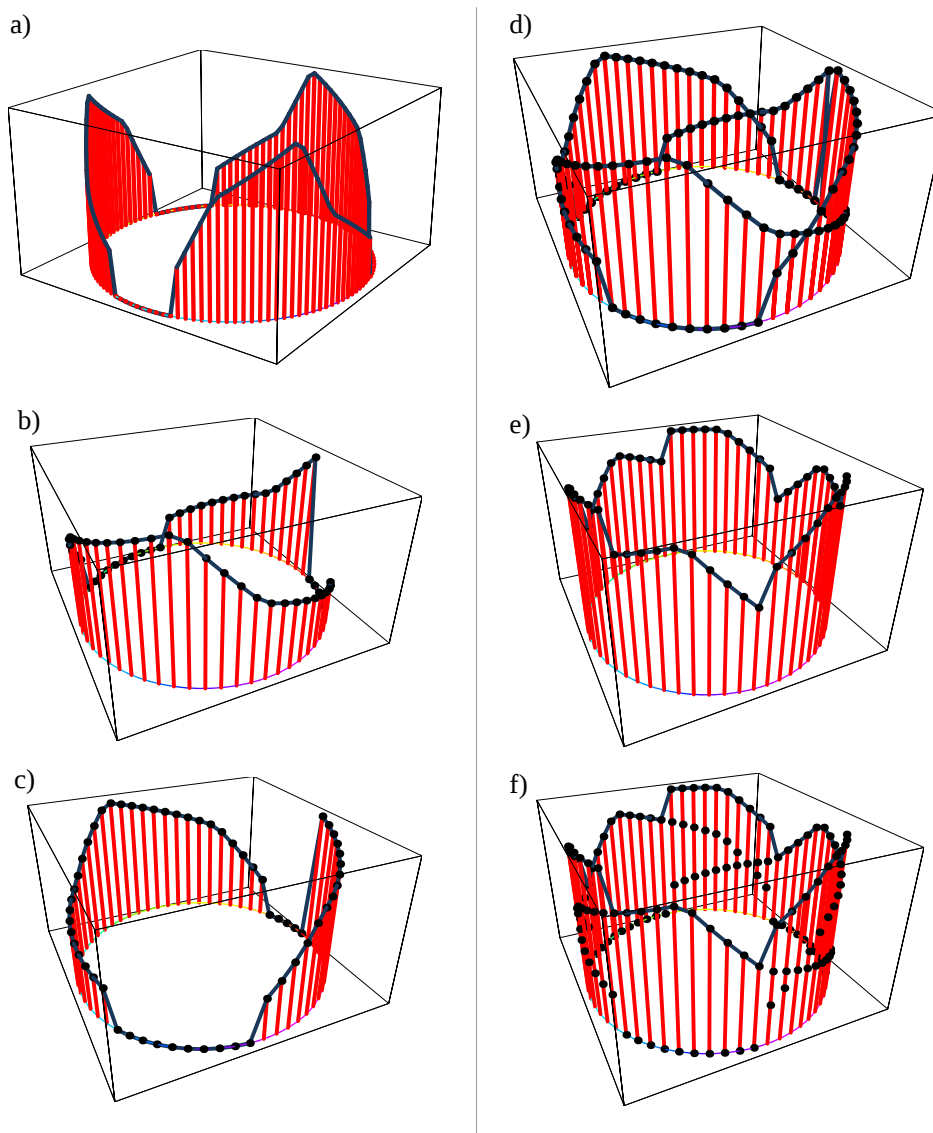
Figure 8.10: Illustration of aliasing in the frequency domain.
