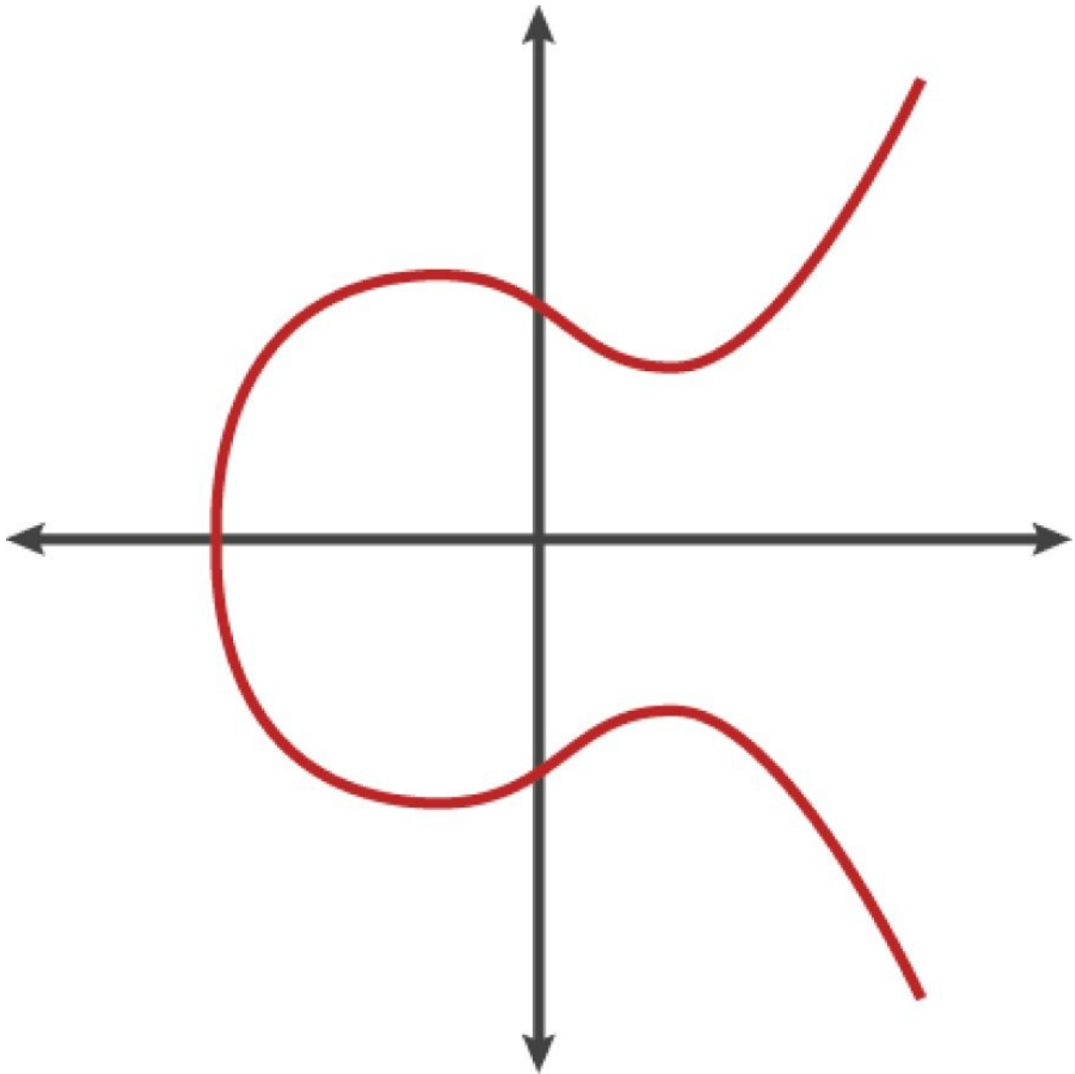
Figure 4-1. A visualization of an elliptic curve
