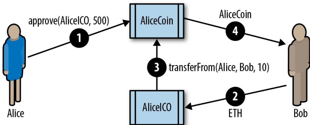
Figure 10-1. The two-step approve & transferFrom workflow of ERC20 tokens
