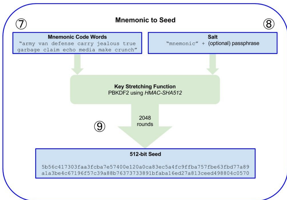
Figure 5-3. From mnemonic to seed
