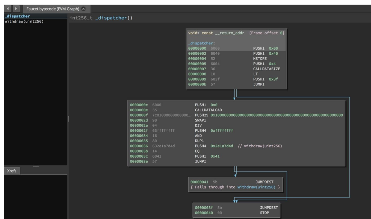
Figure 13-2. Disassembling the Faucet runtime bytecode
