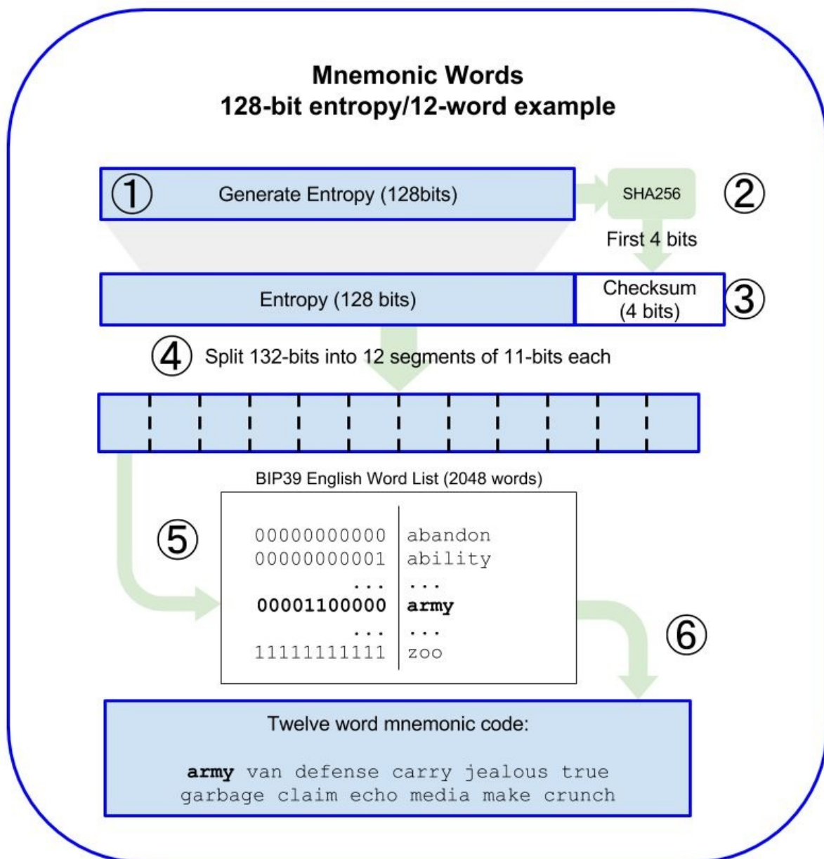
Figure 5-2. Generating entropy and encoding as mnemonic words
