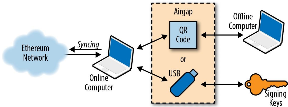
Figure 6-7. Offline signing of Ethereum transactions
