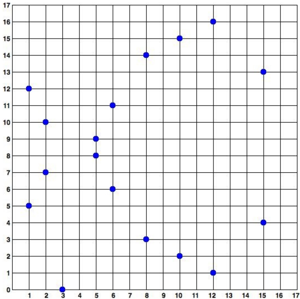
Figure 4-2. Elliptic curve cryptography: visualizing an elliptic curve over F(p) , with p=17
