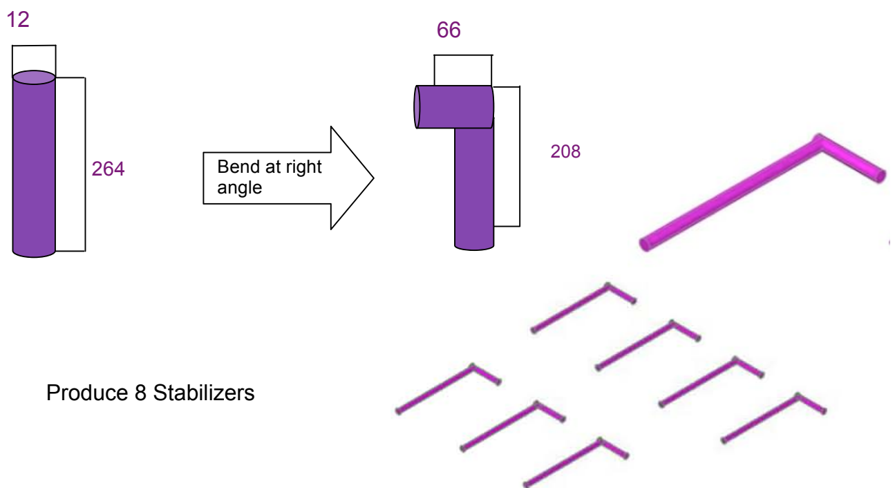
Figure 10.1 Dimensions of the round bar used to produce the pot stabilizer.
