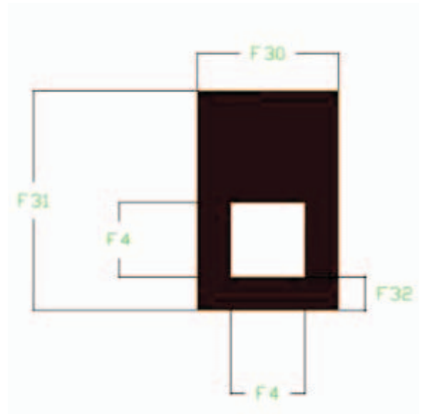
Figure 4.4: Dimension of the front plate of the combustion chamber
