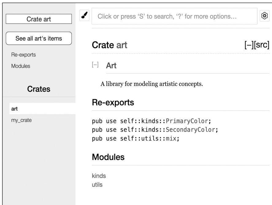
Figure 14-4: The front page of the documentation for art that lists the re-exports
