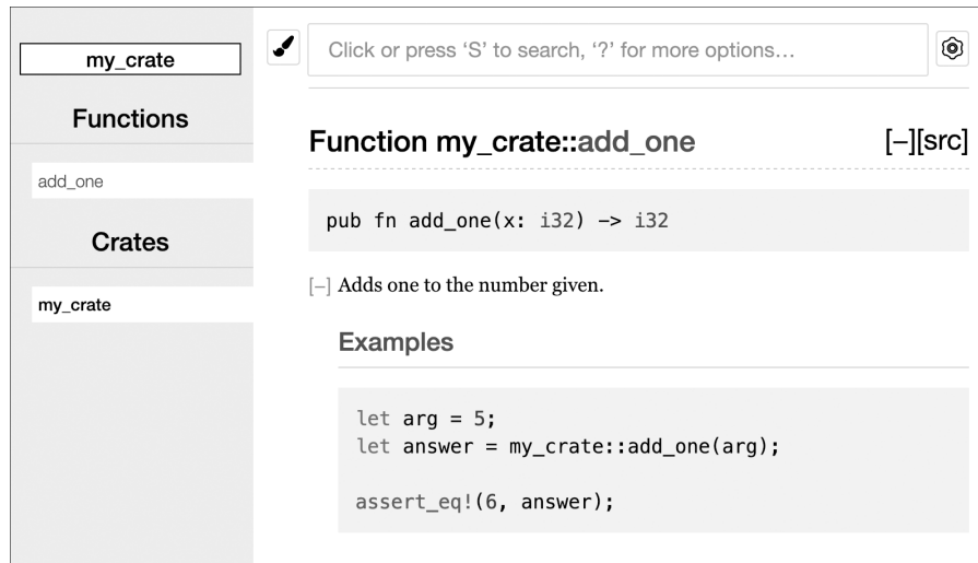
Figure 14-1: HTML documentation for the add_one function
